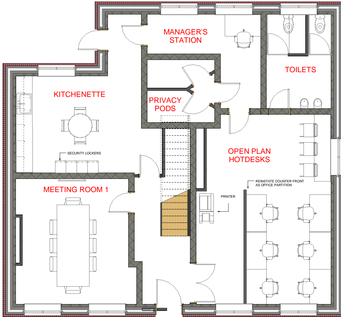
Ground Floor - Architectural Layout SCALE: 1:25
